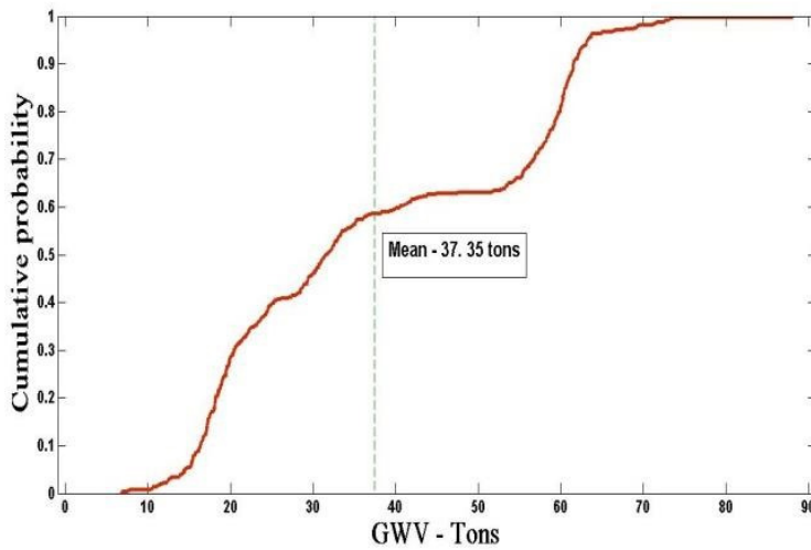
Figure 6. CDF plot of GVW at Peshawarweigh station.
