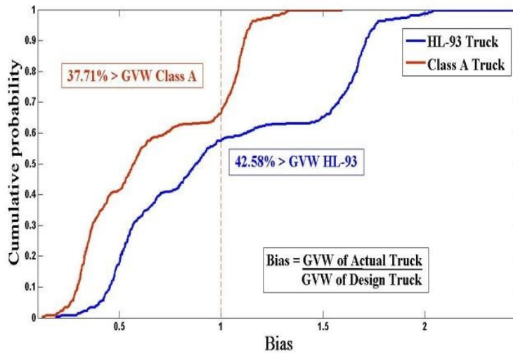
Figure 7. Bias of GVW at Peshawarweigh station.
